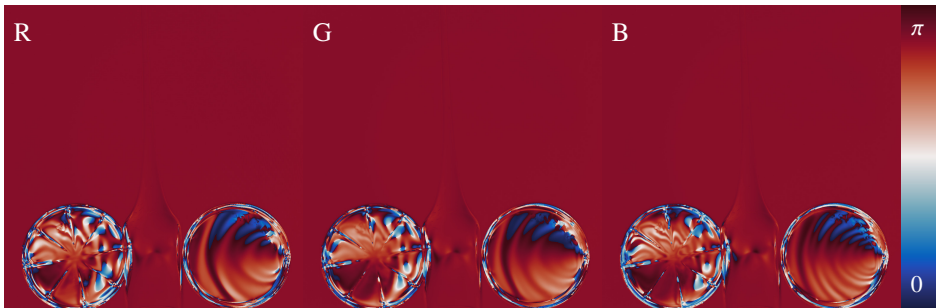
conventional
