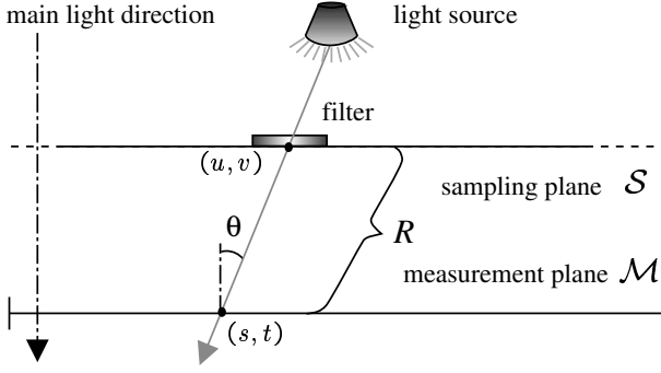
Figure 1. Configuration of the acquisition setup. Light is emitted from the light source, prefiltered on the sampling plane, and recorded on the measurement plane.
